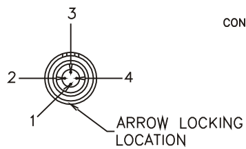
VIEW A-A SHOWN FROM PIN VIEW
